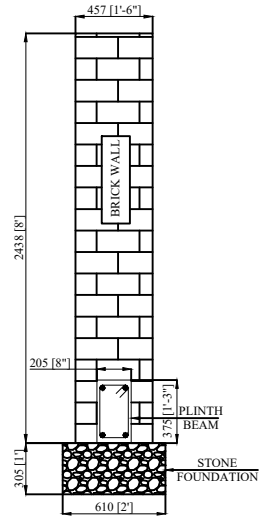
CROSS SECTION
